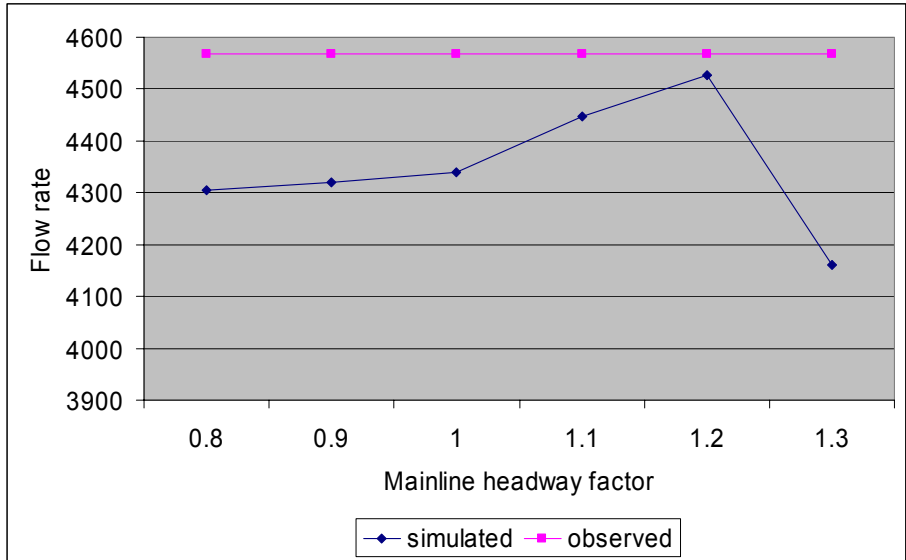
Figure 4 Calibration of headway factor of mainline freeway links
