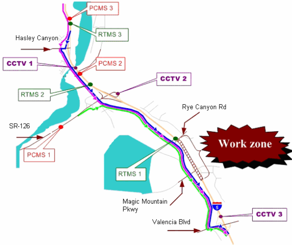
Figure 2 Work zone site with the deployment of the CHIPS system
